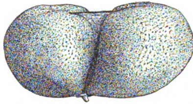
FIG. 146. — A twin-fruit, of Mandarin Orange; \times \frac{1}{2} . (Drawn from a photograph.)
